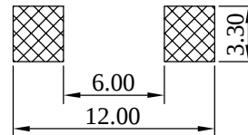
( PCB Pattern )
