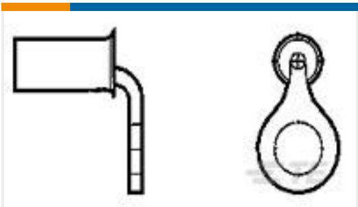
TE Part #184269-1 SOLISTRAND 16-14HD 90 RING 8
