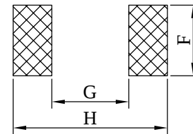
( PCB Pattern )
